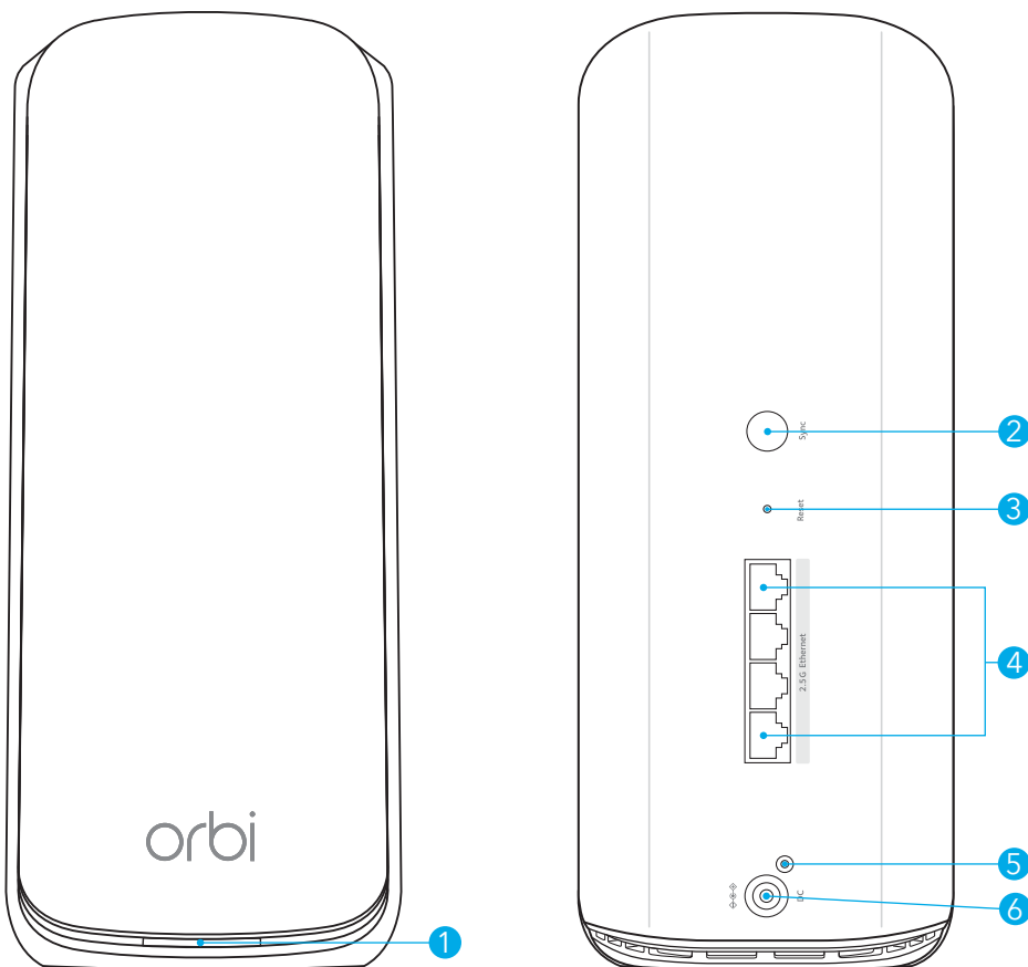
Figure 2. Orbi satellite front (left figure) and back (right figure) views
