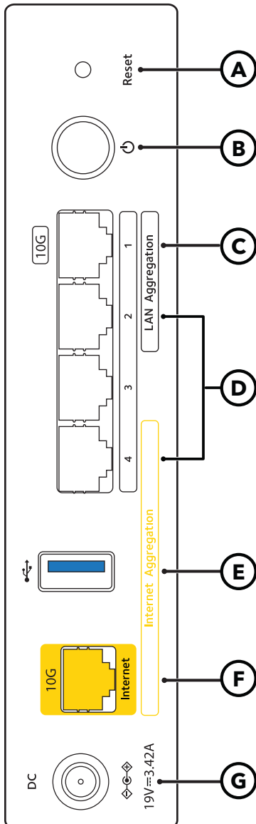
Figure 3. Rear panel
